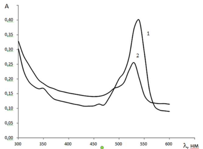
Fig. 2. The spectra of rhodamine and eosine adsorbed into PMM
