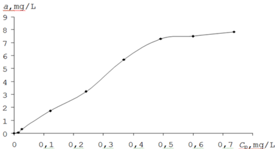
Fig. 3. Adsorption isotherms of eosine adsorbed into PMM
